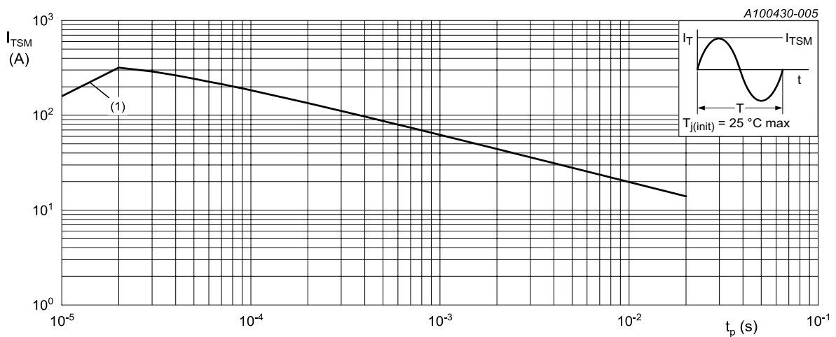
Fig. 3. Non-repetitive peak on-state current as a function of the number of sinusoidal current cycles; maximum values
