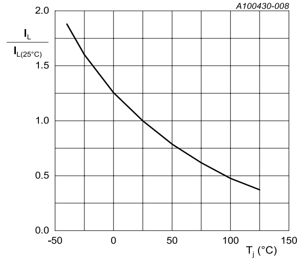
Fig. 7. Normalized latching current as a function of junction temperature
