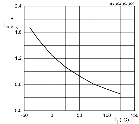
Fig. 8. Normalized holding current as a function of junction temperature
